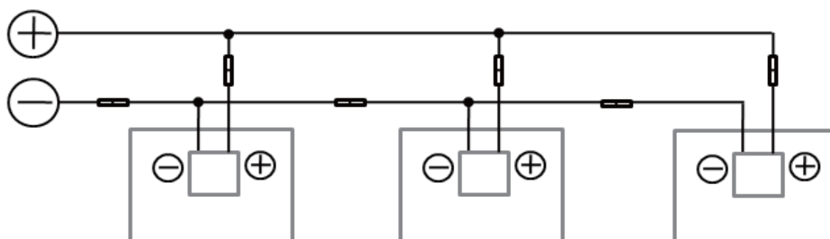
Fig.10-2 Parallel Connection
