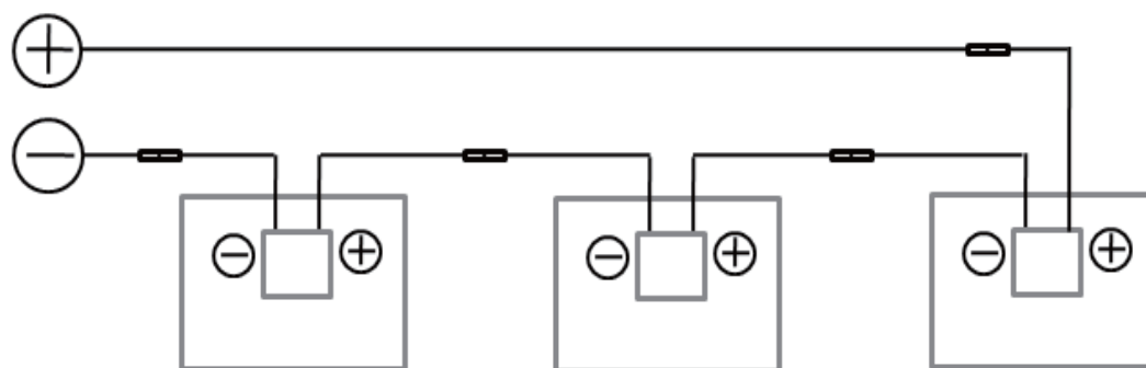
Fig. 10-1 Series Connection
