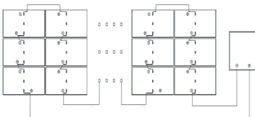
Fig. 9-4 Horizontal installation of long cable modules
