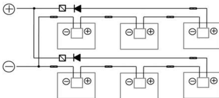
Fig.10-3 Parallel-series Connection
