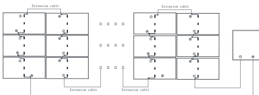
Fig. 9-2 Horizontal installation of short cable modules
